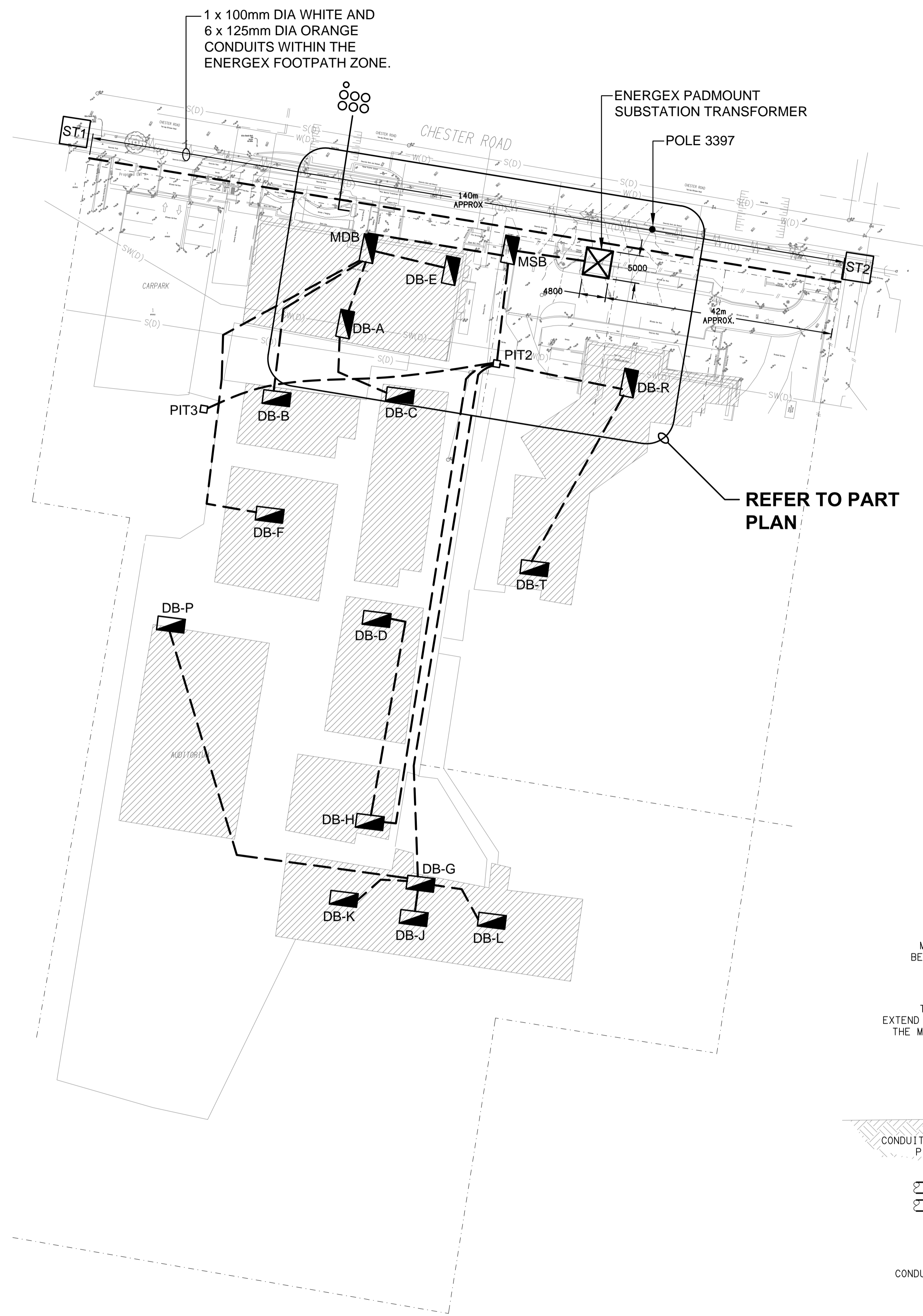
SITE PLAN PROPOSED STAGE 1 DISTRIBUTION SCALE 1:500
