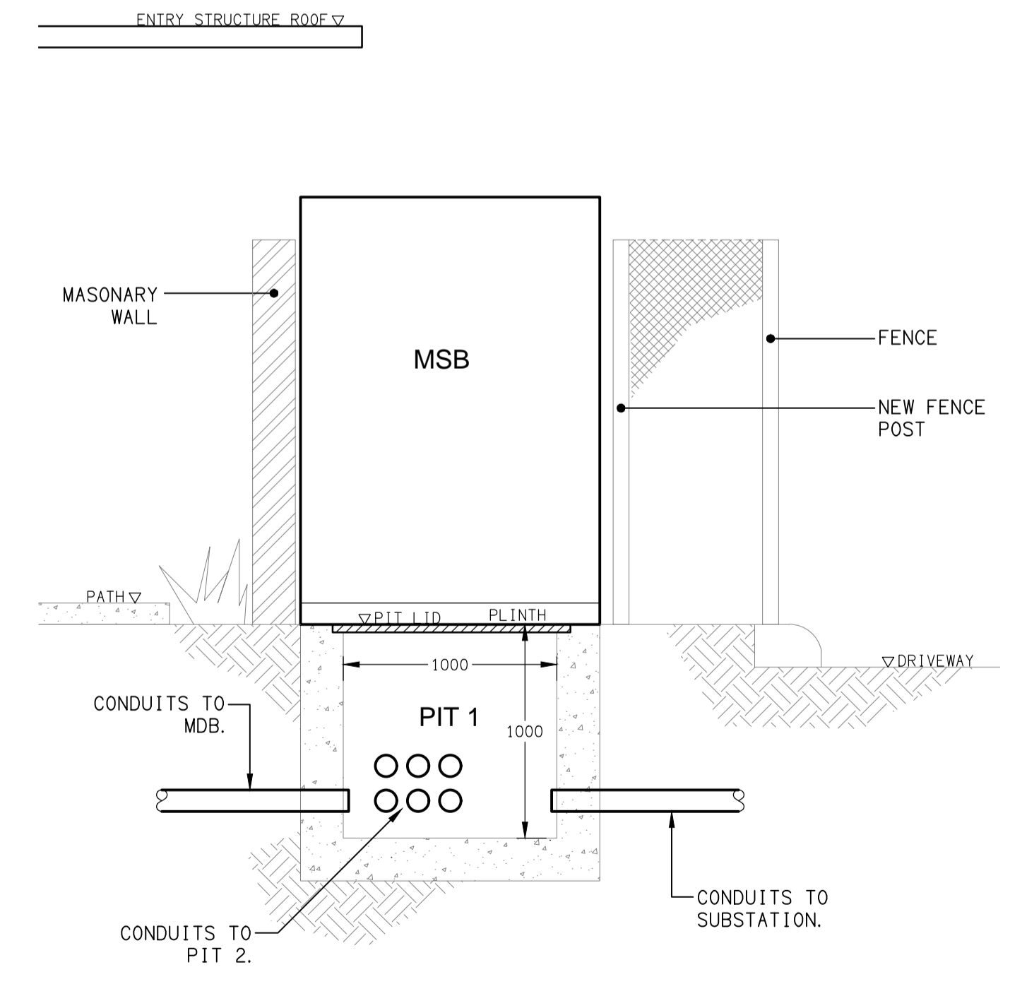
DETAIL B MSB & PIT 1 SECTION NOT TO SCALE
